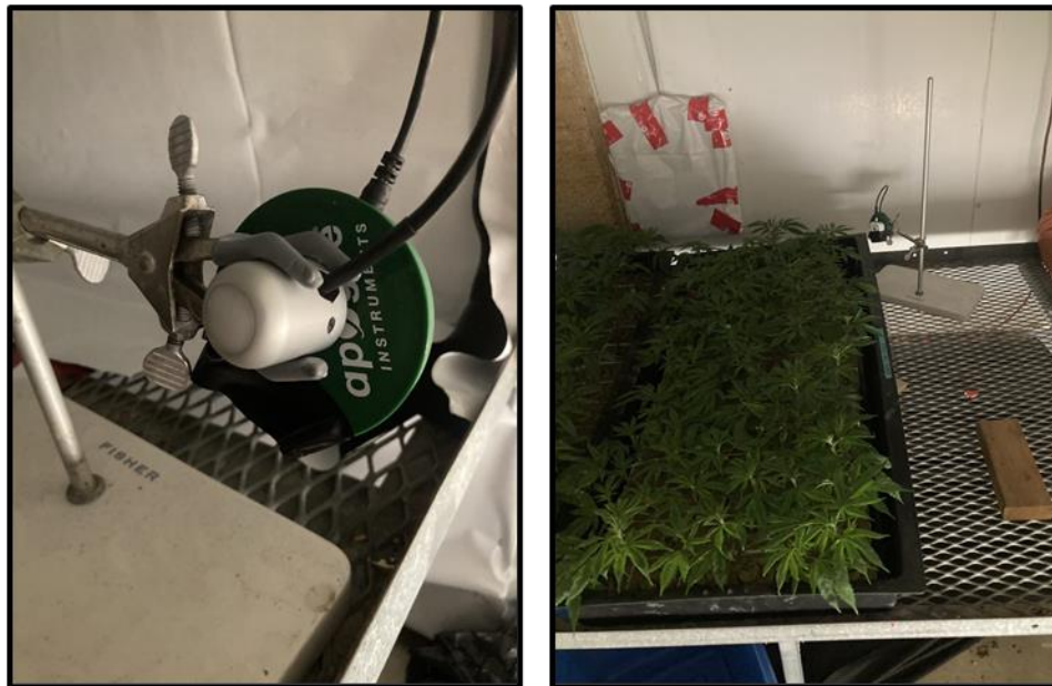
Figure 2 Using the Apogee SQ-640 Light Pollution Sensor and \mu Cache Bluetooth Micro Logger (hidden behind green sensor base) on a retort stand to directionally-characterize stray light pollution in cannabis photoperiod treatment plots.
